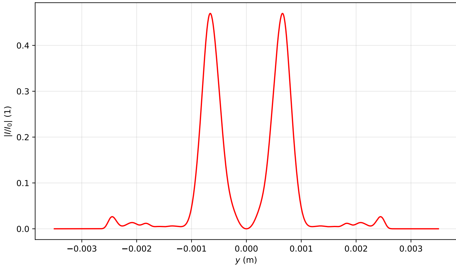
Intensity profile I(x=0, y, z=2.229)/I_0 , \text{Pin}=7.0\text{Pcr} , artificial time
